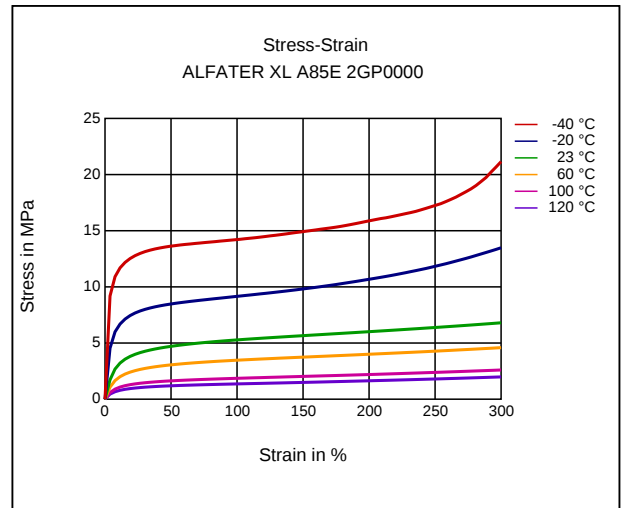
Stress-Strain
